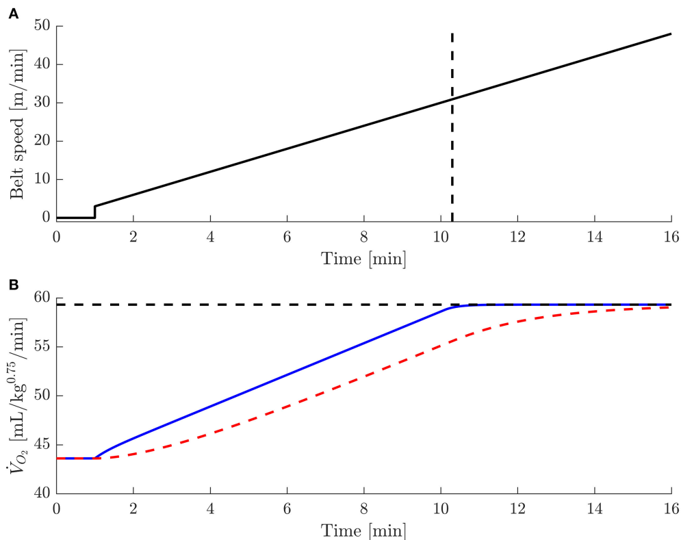
FIGURE 1 | Summary of simulation results of Ayachi2016's ramp 3, 0 degrees protocol. (A) Belt speed against time. The vertical dashed line indicates when the "true" \dot{V}O_2 reaches the value for \dot{V}O_{2peak} calculated from the "measured" \dot{V}O_2 (B). (B) Modeled "true" \dot{V}O_2 (blue, solid curve) and modeled "measured" \dot{V}O_2 (red, dashed curve), calculated from the true \dot{V}O_2 under the assumptions detailed in the text, against time. The horizontal dashed line indicates the assumed value for \dot{V}O_{2max} , which was taken from Ayachi2016.
