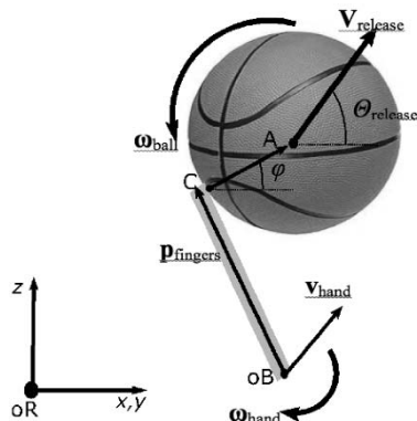
Figure 2 The hand and fingers were modeled as a rigid segment BC and kinematics were calculated at t_{release} . The ball was released from point C with velocity v_{release} , angle \theta_{release} , angular velocity \omega_{ball} and angle \phi .
