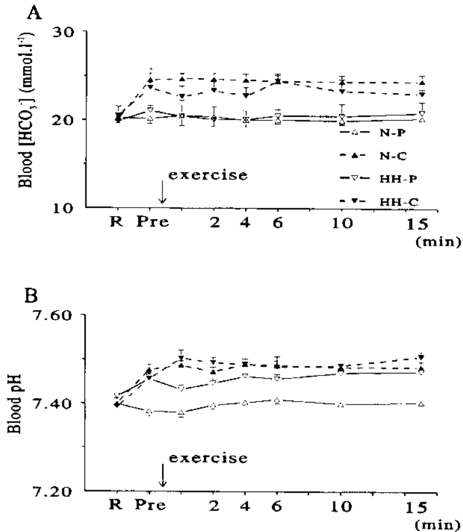
Fig. 1 Changes in blood bicarbonate concentrations ( A ) and in pH ( B ) at rest before treatment ( R ), before prolonged static contraction ( Pre ), and during recovery (mean and SD). N-P Placebo ingestion and exercise during normoxia, N-C sodium citrate ingestion and exercise during normoxia, HH-P placebo ingestion and exercise during acute hypobaric hypoxia, HH-C sodium citrate ingestion and exercise during acute hypobaric hypoxia. After treatment, blood [HCO_3^-] values for N-C and HH-C were significantly greater than for N-P and HH-P , respectively. After treatment, blood pH values for N-C were significantly greater than for N-P . During recovery up to 6th min, blood pH values for HH-C were significantly greater than for HH-P
