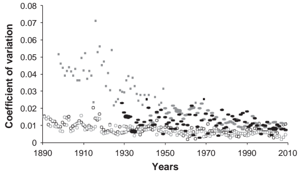
Fig. 2 Coefficient of variations of 10 best performers in thoroughbred (1899–2009; grey squares), greyhounds (1929–2009; black squares), human 200- to 400-m races (1891–2009; grey open circles) and humans 800- to 1500-m races (1891–2009; black open circles).
