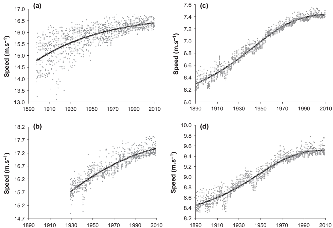
Fig. 1 Models fitting for speed progression ( \text{m s}^{-1} ) between 1891 and 2009, in (a) 10 best thoroughbred performers ( R^2 = 0.56 ); (b) 10 best greyhound performers on short ring races ( R^2 = 0.81 ); (c) Mean speed of the 10 best human performers on 200- to 400-m track races ( R^2 = 0.97 ); (d) Mean speed of the 10 best human performers on 800- to 1500-m track races ( R^2 = 0.94 ). The calculated a , b , c , d parameters of the Gompertz function were for thoroughbred (respectively, 77.8, 3.77, 0.46, 16.59), greyhound (respectively, 14.99, 1.99, 0.60, 17.7), 800- to 1500-m human races (respectively, 1.45, 0.26, 3.06, 7.44) and for 200- to 400-m human races (respectively, 1.29, 0.20, 3.31, 9.52).
