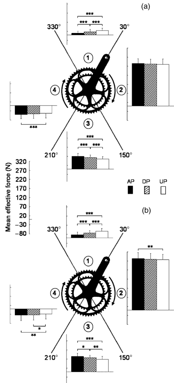
Fig. 3. Mean values of effective force calculated for four angular sectors as a function of crank position over the complete cycle in the three body configurations [(a) at VT1D20% and (b) at respiratory compensation point (RCP)]. Sector 1, 330–30°; Sector 2, 30–150°; Sector 3, 150–210° and Sector 4, 210–330°. AP, aero posture; DP, dropped posture; UP, upright posture. *** P < 0.001 , ** P < 0.01 , * P < 0.05 significant difference between two conditions.
