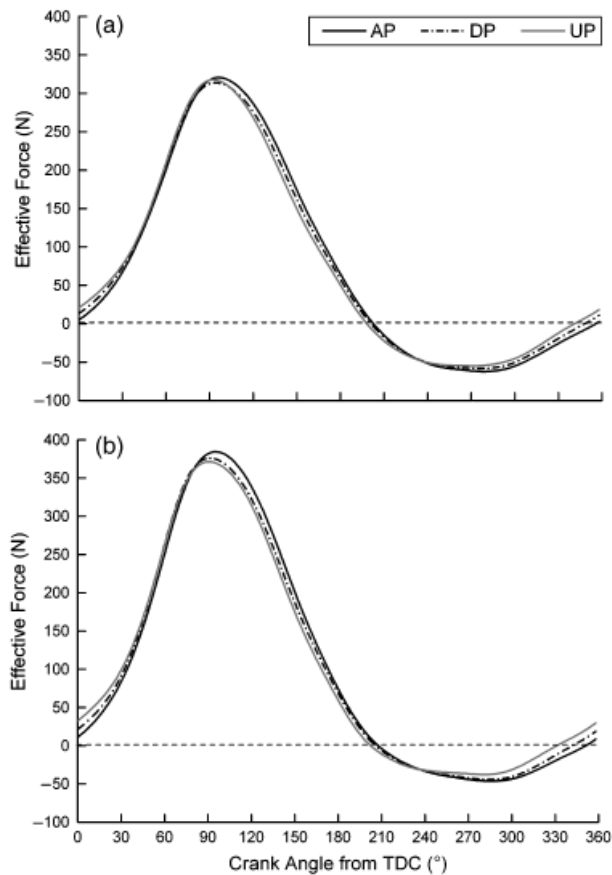
Fig. 2. Mean profile of the effective pedal force measured during the exercises at VT1D20% (a) and respiratory compensation point (RCP) (b) in the three upper body positions for the entire population. AP, aero posture; DP, dropped posture; UP, upright posture. Note the higher peak value of force produced during the second part of the downstroke phase and the lower value during the last part of the upstroke and the beginning of the downstroke for AP compared with UP.
