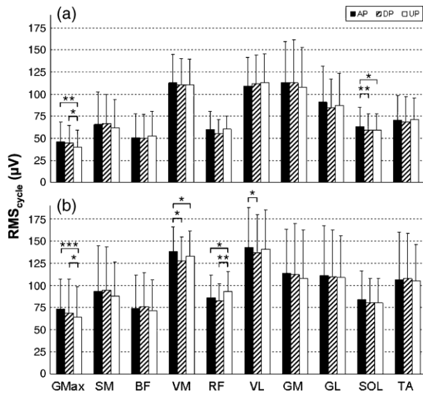
Fig. 4. Mean values of the root mean squared (RMS) magnitude for the complete cycle ( RMS_{cycle} , i.e. 0 to 3601) for the three body positions (AP, aero posture; DP, dropped posture; UP, upright posture) at both constant submaximal power outputs [VT1D20% and respiratory compensation point (RCP)] for 10 lower limb muscles implied in pedalling. GMax, gluteus maximus ; SM, semimembranosus , BF, Biceps femoris ; VM, vastus medialis ; RF, rectus femoris ; VL, vastus lateralis ; GM, gastrocnemius medialis ; GL, gastrocnemius lateralis ; SOL, soleus and TA, tibialis anterior .
