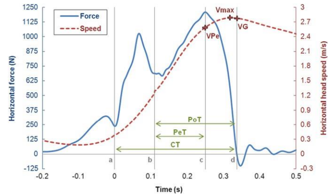
Fig. 5. Mean horizontal component of the force applied on the turning wall and mean horizontal speed of the head for the ten elite swimmers. Vertical gray lines point out the first contact (a), the end of placement (b), the force peak (c), and the end of push-off (d). CT, PeT and PoT are durations between these key times. VPe, Vmax and VG are selected horizontal speeds.
