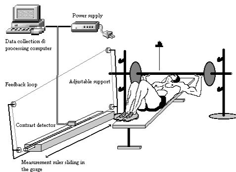
Fig. 1 Schematic diagram of the acquisition equipment and set-up used for evaluating an athlete on a bench exercise.
