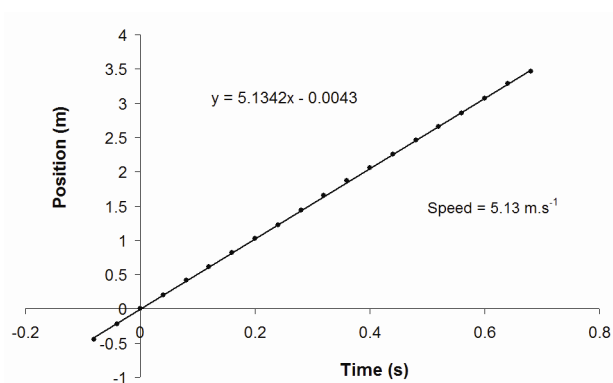
Figure 3: Example of horizontal position of the CM in the referential of the camera, and calculus of the speed of the CM of the runner.
